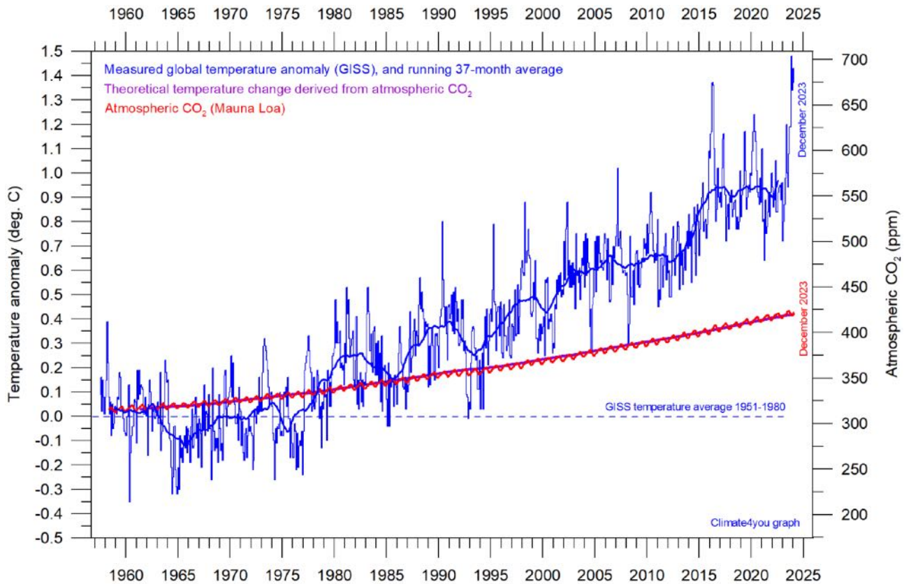
Diagrams showing UAH, RSS, HadCRUT5, NCD and GISS monthly global air temperature estimates (blue) and the monthly atmospheric CO 2 content (red) according to the Mauna Loa Observatory , Hawaii. Purple line (running along red CO 2 curve) shows theoretical temperature change due to changing atmospheric CO 2 . The Mauna Loa data series begins in March 1958, and 1958 was therefore chosen as starting year for all diagrams above. Reconstructions of past atmospheric CO 2 concentrations (before 1958) are not incorporated in this diagram, as such past CO 2 values are derived by other means (ice cores, stomata, or older measurements using different methodology), and therefore are not directly comparable with direct atmospheric measurements.
