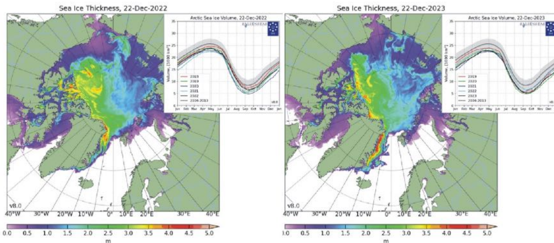
Diagrams showing Arctic sea ice extent and thickness 22 December 2022 (left) and 2023 (right and above) and the seasonal cycles of the calculated total arctic sea ice volume, according to The Danish Meteorological Institute (DMI) . The mean sea ice volume and standard deviation for the period 2004-2013 are shown by grey shading. Please note that DMI on 7 December 2021 changed their sea ice calculation model. DMI's description of the model version change can be read here: http://polarportal.dk/en/sea-ice-and-icebergs/sea-ice-thickness-and-volume/
