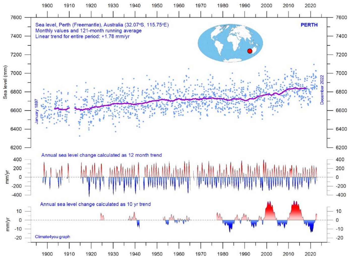
Perth (Freemantle, SW Australia) monthly tide gauge data from PSMSL Data Explorer . The blue dots are the individual monthly observations, and the purple line represents the running 121-month (ca. 10 yr) average. The two lower panels show the annual sea level change, calculated for 1 and 10 yr time windows, respectively. These values are plotted at the end of the interval considered. Last month shown: December 2022.
