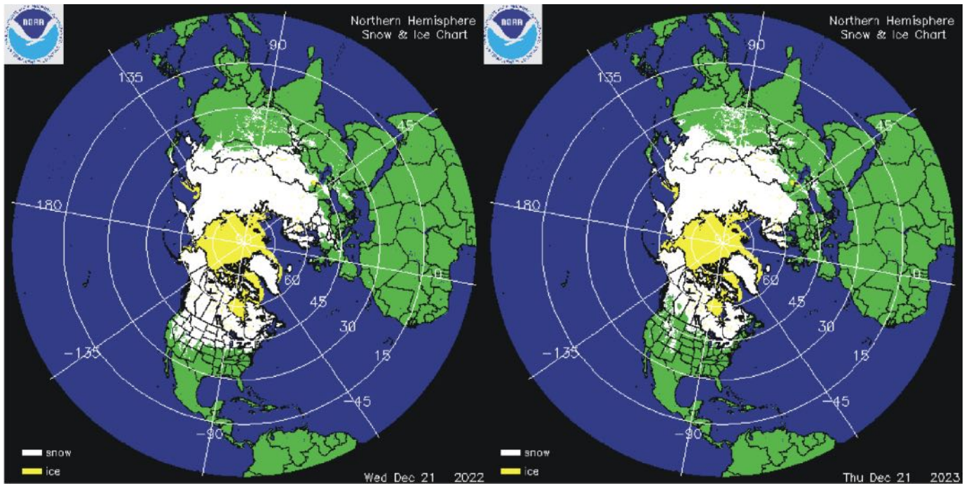
Northern hemisphere snow cover (white) and sea ice (yellow) 21 December 2022 (left) and 2023 (right). Map source: National Ice Center (NIC) .
