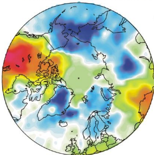
Surface air temperature December 2023 versus December 2022
