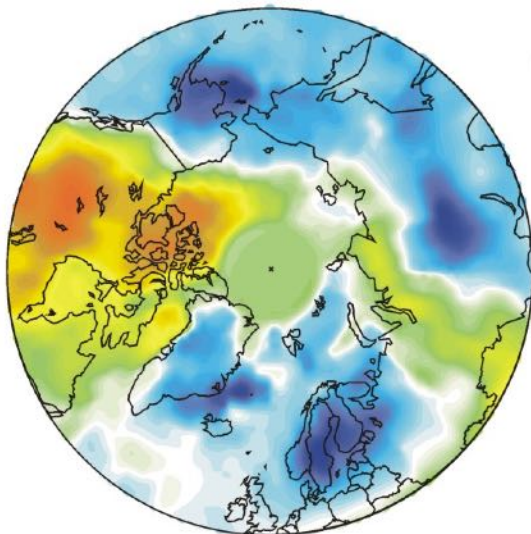
Surface air temperature December 2023 versus December last 10 yr
