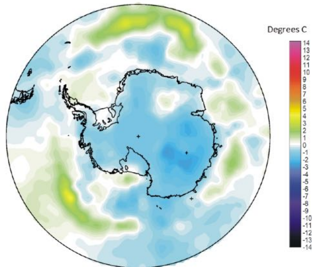
Surface air temperature December 2023 versus December last 10 yr
