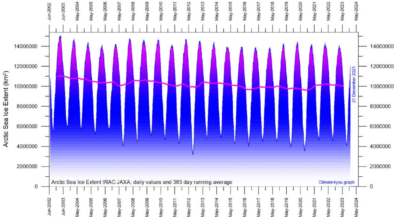
Diagram showing daily Arctic sea ice extent since June 2002, to 21 December 2023, data courtesy of Japan Aerospace Exploration Agency (JAXA) .
