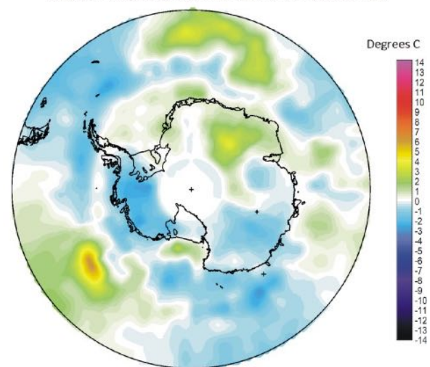
Surface air temperature December 2023 versus December 2022
