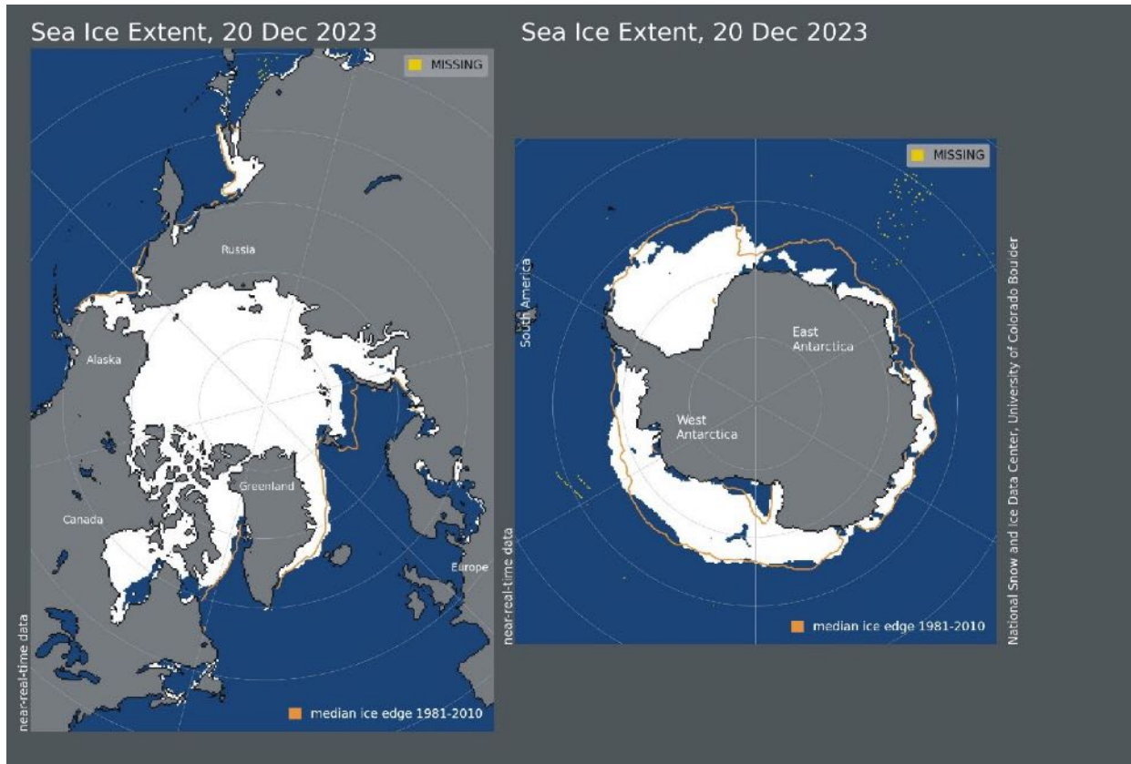
Sea ice extent 20 December 2023. The median limit of sea ice (orange line) is defined as 15% sea ice cover, according to the average of satellite observations 1981-2010 (both years included). Sea ice may therefore well be encountered outside and open water areas inside the limit shown in the diagrams above. Map source: National Snow and Ice Data Center (NSIDC).
