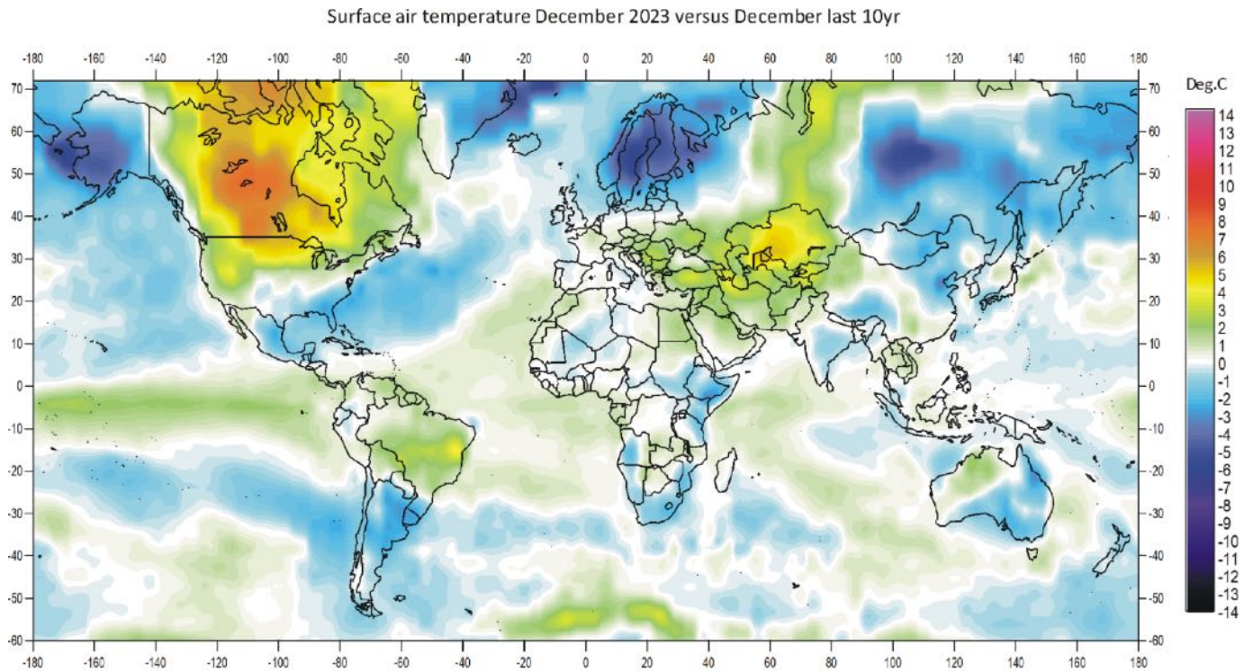
Surface air temperature December 2023 versus December last 10 yr
